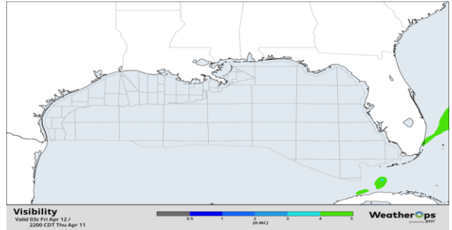
Visibility Forecast 0900 CT Apr-12
