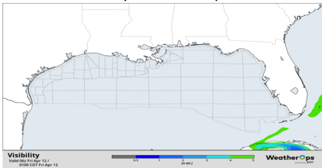
Visibility Forecast 1200 CT Apr-12
