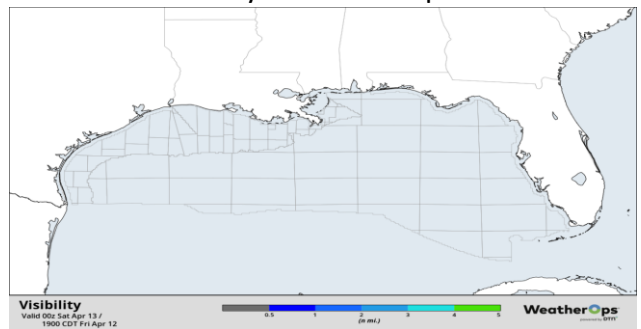
Visibility Forecast 0600 CT Apr-13
