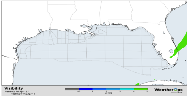
Visibility Forecast 0600 CT Apr-12
