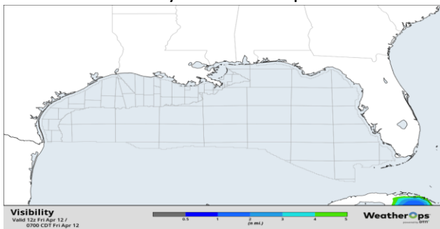
Visibility Forecast 1800 CT Apr-12
