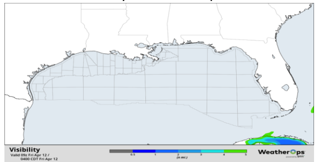
Visibility Forecast 1500 CT Apr-12
