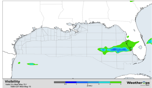
Visibility Forecast 1500 CT May-15
