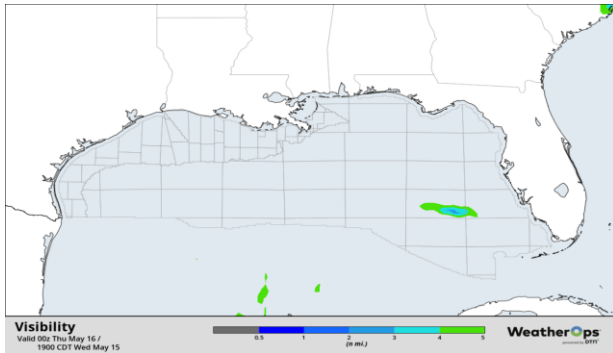
Visibility Forecast 1800 CT May-15
