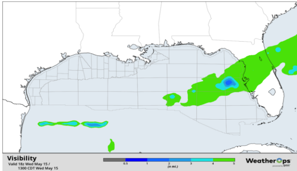
Visibility Forecast 1200 CT May-15
