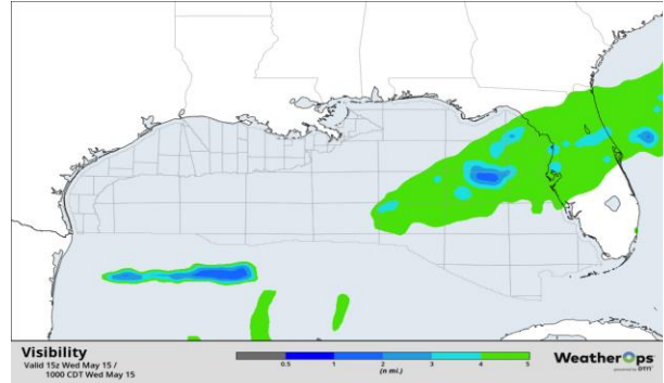
Visibility Forecast 0900 CT May-15
